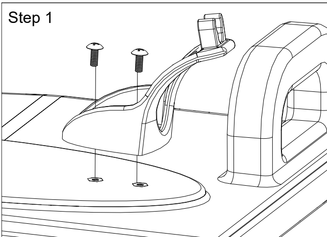
Step 1 Attach the (2) Hose Wraps to the top of the tank with (4) Phillips Head Screws
