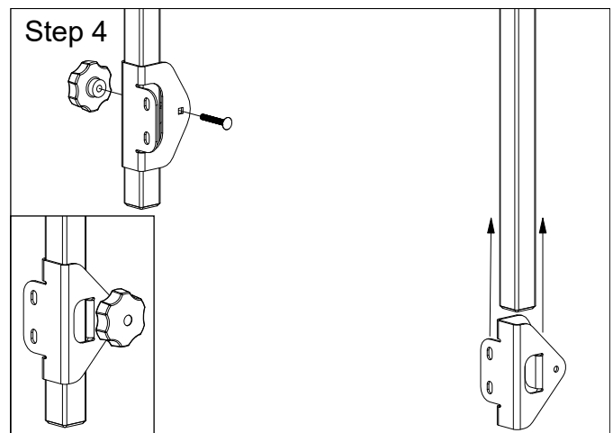
Step 4 Slide the boom clamps up the boom mount tubes and install the 1/4" carriage bolt and Lobe Knob., make sure the boom clamps are installed with the square carriage bolt holes or two boom mount holes to the inside and the lobe knob to the outside.
