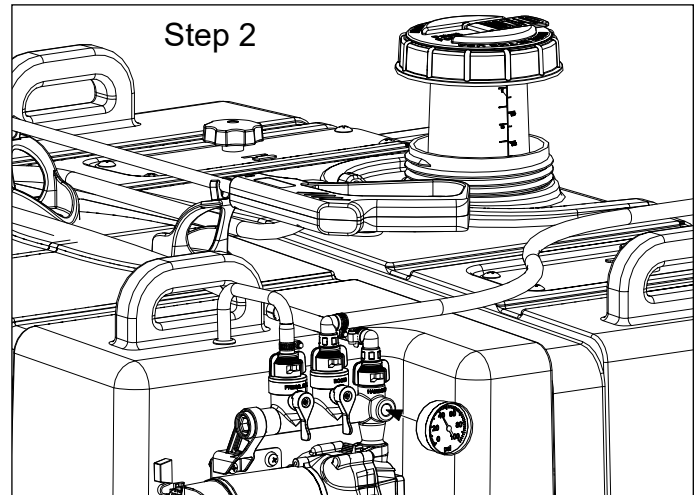
Step 2 Thread Pressure Gauge into open port on manifold, as shown. Thread Multi-Lid on to tank.
