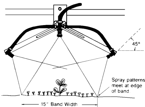
THREE NOZZLES PER 30 " OR 40 " ROW SPACING
